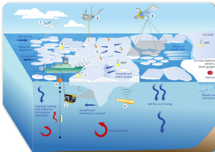
FIGURE 3 | Observing system for sea ice includes: drifting buoys (a); ice-deformation arrays (b); mass-balance- and snow-buoys (c); wave buoys (d); autonomous underwater (e); airborne vehicles (f); satellite altimeters; and radars and radiometers (g); ships (h); underway and in situ sea-ice sampling (i) and ROVs (j). From Newman et al., 2019 .
