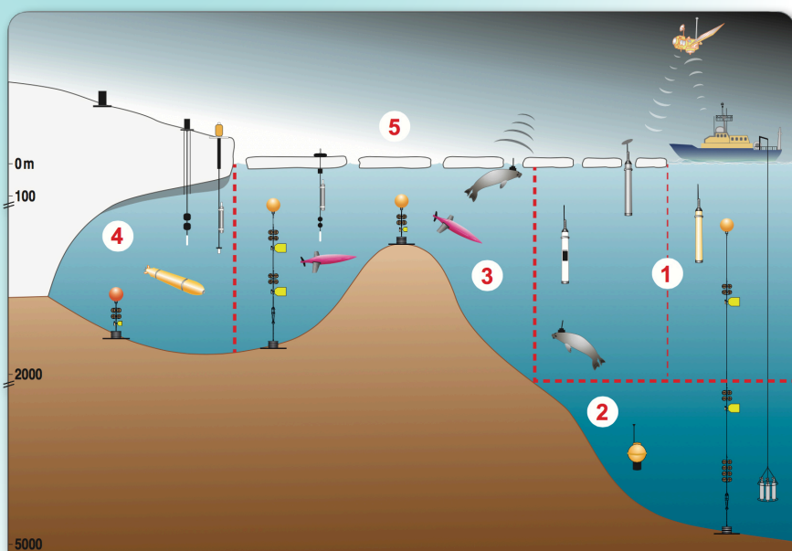
FIGURE 2 | The high latitude Southern Ocean and Antarctic margin includes several physical environments (1-5), each with distinct characteristics that mean a different mix of platforms is needed to observe each one. 1: Open ocean shallower than 2000m depth, 2: Deep ocean, 3: Continental shelf and slope, 4: Ice shelf cavities, 5: Sea ice and ice-ocean-atmosphere interaction (from "Seeing Below the Ice: A strategy for observing the ocean beneath Antarctic sea ice and ice shelves" , 2014, SOOS report, 57 pp).
